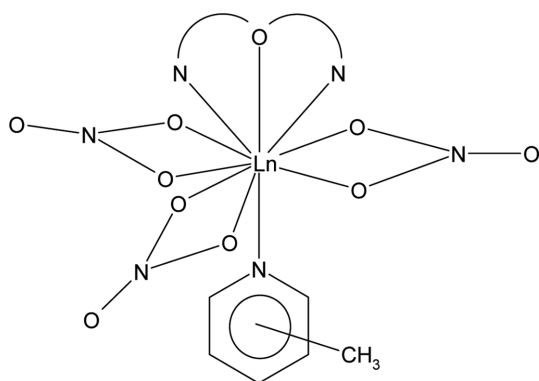
Fig. 2. Proposed structure of [Ln(FFAAPS)(NO_3)_2(\gamma\text{-Pic})] , Ln = La, Pr, Nd, Sm, Gd, Tb, Dy or Ho) and Pic = \alpha -, \beta - or \gamma -picolines (C.N. = 10).
