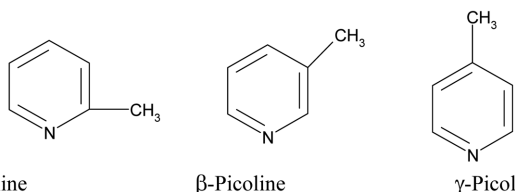
Fig. 1. Structures of 4[N-(furfural)amino]antipyridine semicarbazone (FFAAPS) and \alpha -, \beta - and \gamma -picolines.
