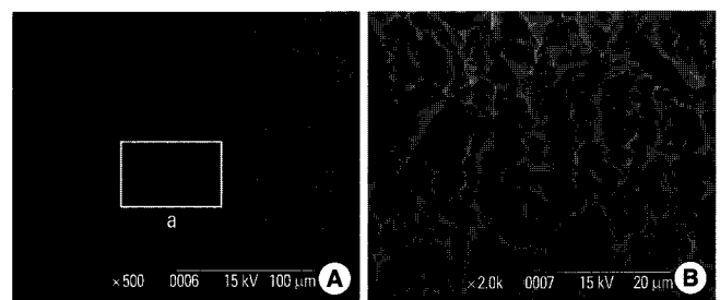
Figure 6. (A) Sand-blasted, large grit, acid-etched implant surface irradiated at 140 mJ/pulse for 1.5 minutes ( \times 500 ). (B) Inset of Figure 6A. Flattened surface is observed ( \times 2,000 ).
