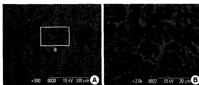
Figure 10. (A) Sand-blasted, large grit, acid-etched implant surface irradiated at 180 mJ/pulse for 2 minutes ( \times 500 ). (B) Inset of Figure 10A. Flattened surface is observed ( \times 2,000 ).
