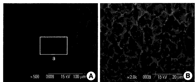
Figure 7. (A) Sand-blasted, large grit, acid-etched implant surface irradiated at 140 mJ/pulse for 2 minutes ( \times 500 ). (B) Inset of Figure 7A. Flattened surface is observed ( \times 2,000 ).
