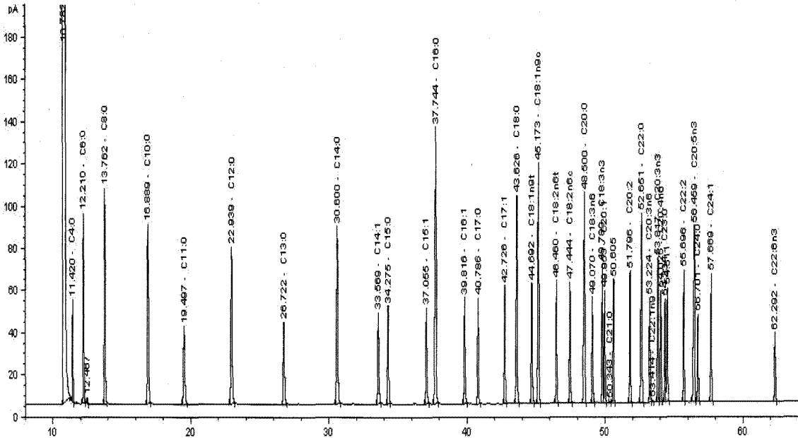
Fig. 1. Chromatogram of fatty acid standard by GC-FID.
