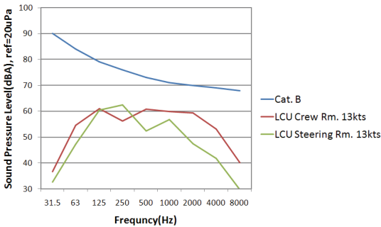
Fig. 6 Measured indoor noise of LCU
