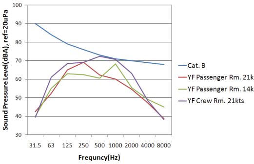
Fig. 2 Measured indoor noise of YF
