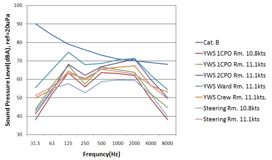
Fig. 8 Measured indoor noise of YWS
