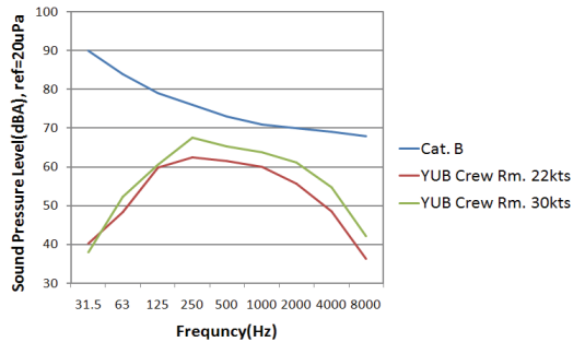
Fig. 4 Measured indoor noise of YUB
