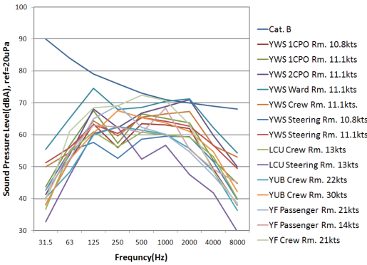
Fig. 9 Overall of measured indoor noise
