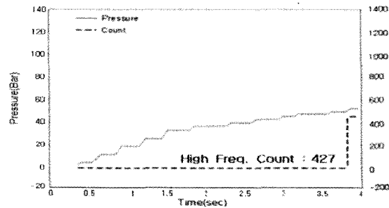
(b) sandwich cylinder
