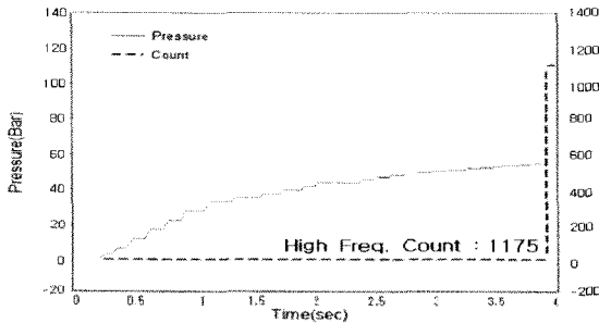
(b) sandwich cylinder
