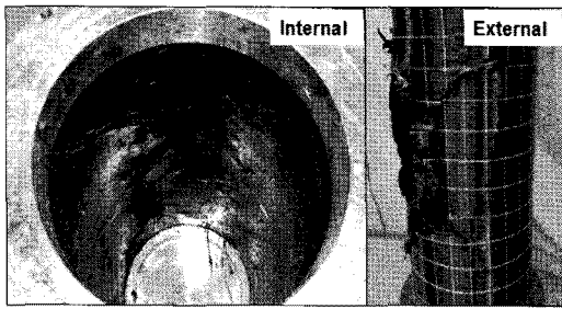
(a) Filament wound composite cylinder
