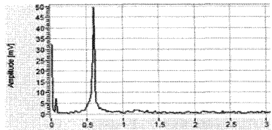
Fig. 6 FFT analyses of the AE signals under the impact test.
