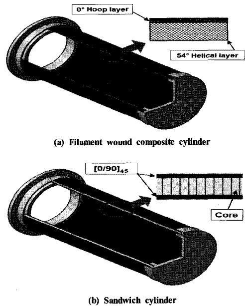
Fig. 3 Shapes of composite cylinder.
