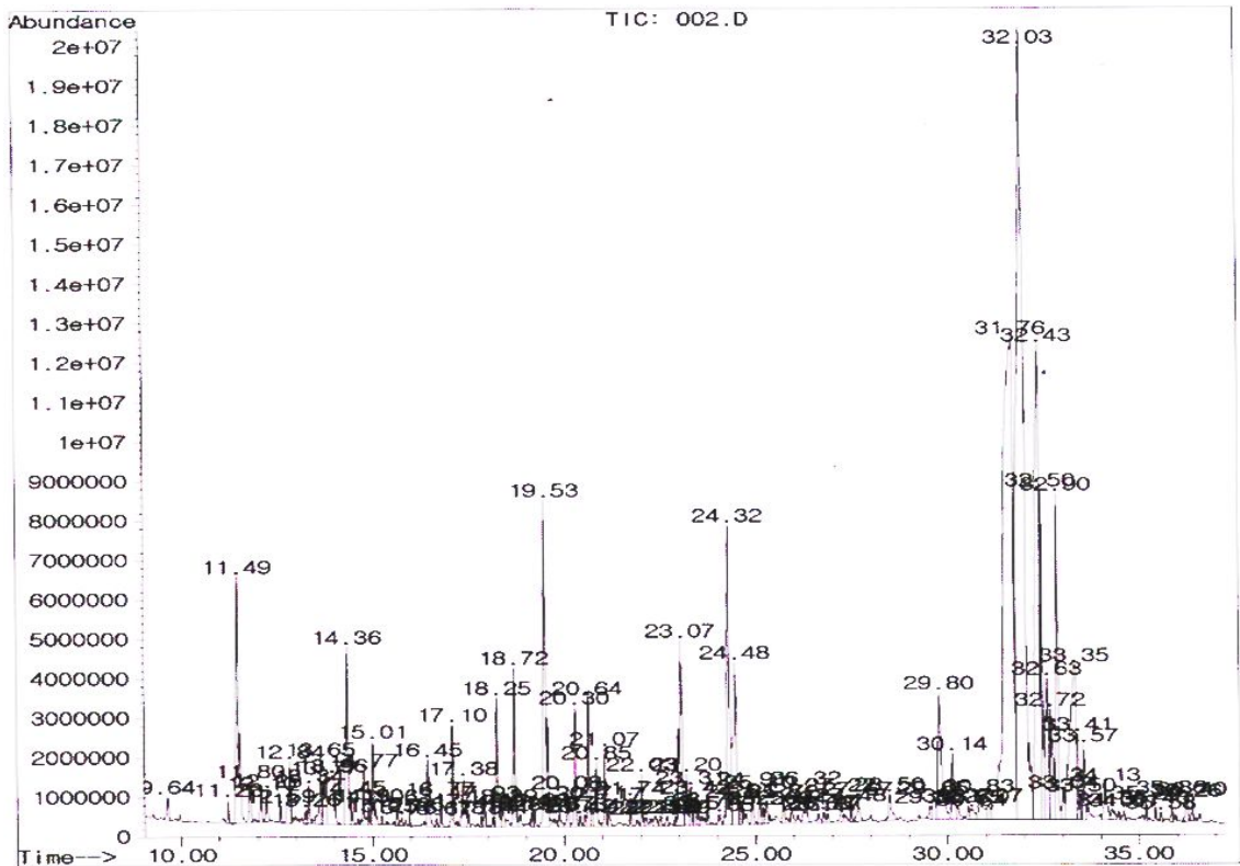
Fig. 1. A chromatogram of a patient. The number on a peak is the retention time of that peak.
