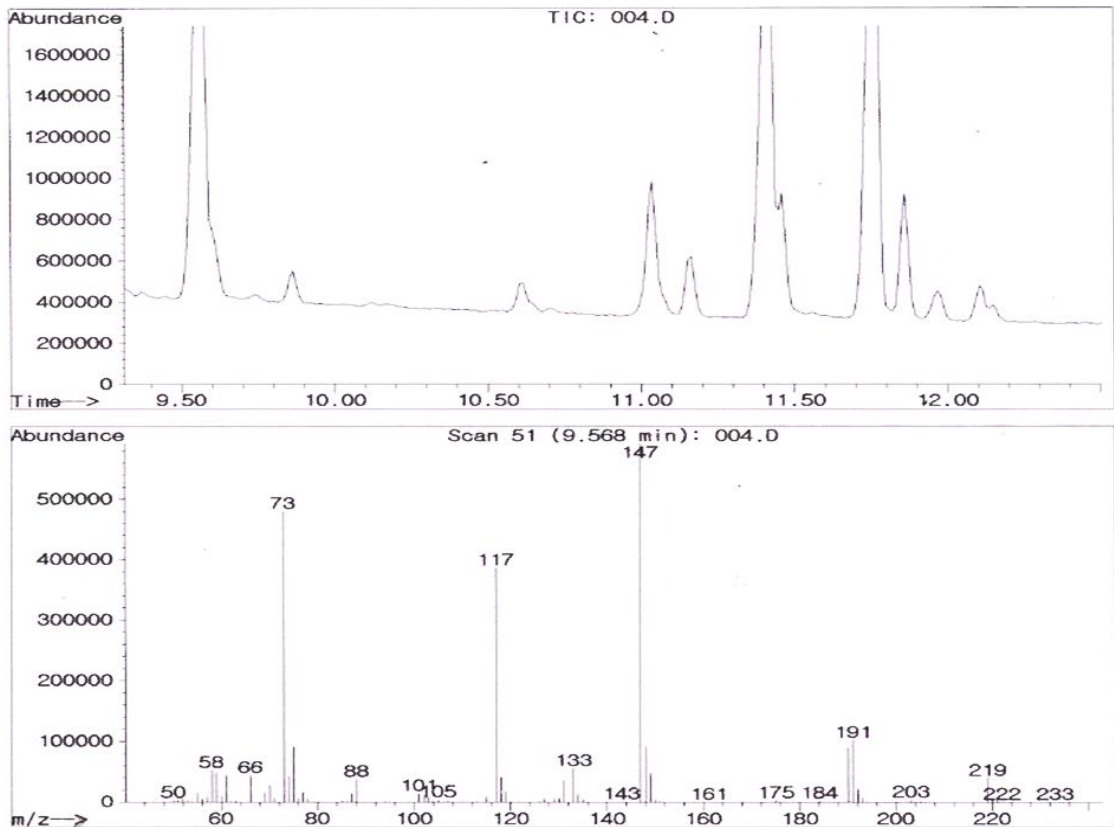
Fig. 2. A part of chromatogram and mass spectrum of 9.568 peak(lactic acid). The number on mass spectrum is molecular weight of each fragments.
