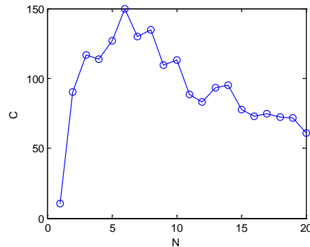
Fig. 5. The cost function C for a training subset from CAMERA database with an embedding rate of 50%, using the threshold selection procedure. The performance peaks at N_p = 6 .
