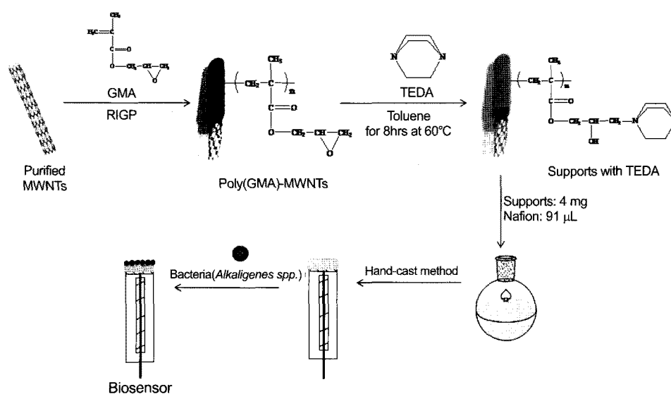
Scheme 1. Preparation procedure of the electrochemical microbial biosensor (EMB) based on MWNT supports with amine groups by RIGP.
