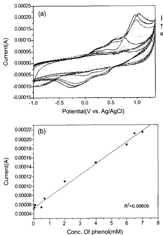
Figure 5. Cyclic voltammograms of the EMB in a 0.1 M phosphate buffer solution (pH=7.0) containing different phenol concentration (a) (from a to j: 0, 0.05, 0.1, 0.5, 0.7, 2, 4, 6, 6.5, 7.0 mM) with a scan rate of 100 mV/s and calibration plot of the concentration of phenol with respect to the current (b).
