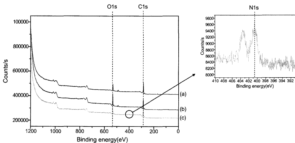
Figure 1. XPS survey scan spectra of the purified MWNTs: (a) poly(GMA)-MWNTs; (b) MWNTs with TEDA; (c) prepared by RIGP.
