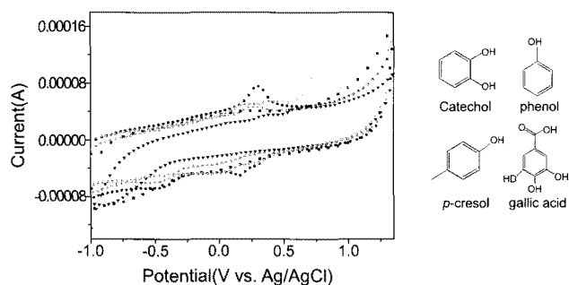
Figure 4. Cyclic voltammograms of the EMB with regards to various phenolic compounds in 0.1 M phosphate buffer solution (■) containing 1 mM catechol (●), 1 mM p -cresol (▼), 1 mM gallic acid (▲), and 1 mM phenol (◆) with a scan rate of 100 mV/s.
