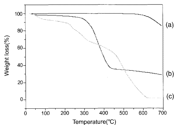
Figure 3. TGA curves of the purified MWNTs (a); poly(GMA)- g -MWNTs (b); MWNTs with TEDA (c).
