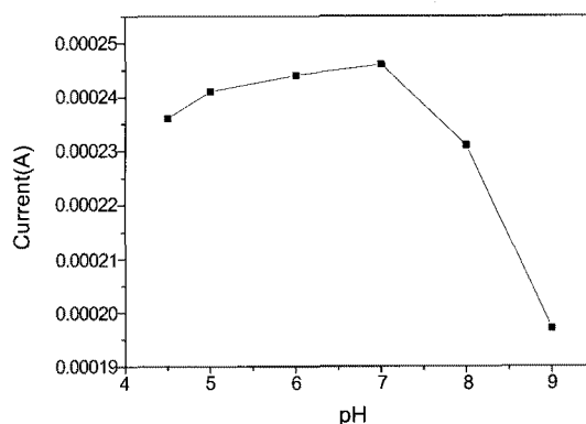
Figure 6. Effect of pH on the response of the EMB in a 0.1 M phosphate buffer solution (pH=4.5, 5, 6, 7, 8, and 9) containing 5 mM phenol at a scan rate of 100 mV/s.
