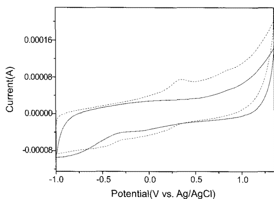
Figure 7. Cyclic voltammograms of the EMB in a 0.1 M phosphate buffer solution (solid line) containing 100 \mu L of red wine (AMOR) (dashed line) with a scan rate of 100 mV/s.
