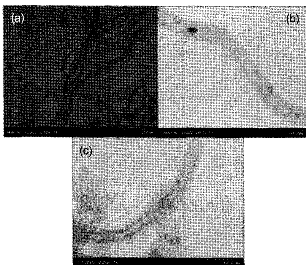
Figure 2. TEM images of the purified MWNTs (a); poly(GMA)- g -MWNTs (b); MWNTs with TEDA (c).
