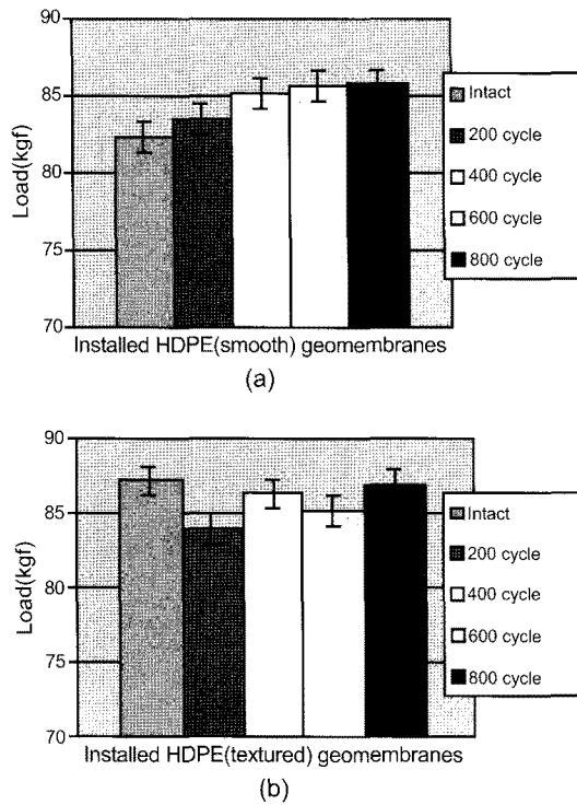
Figure 7. Comparison of puncture resistance of GMs at different loading cycles: (a) HDPE smooth GMs; (b) HDPE textured GMs.
