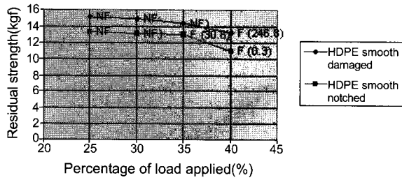
Figure 10. Residual strength of HDPE smooth GMs(notched and damaged) after stress cracking observation at pH 4.
