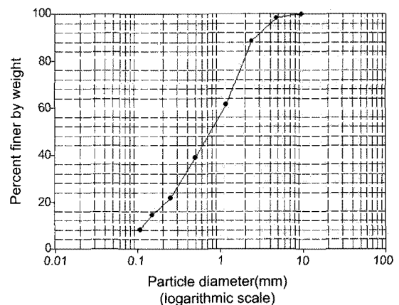
Figure 2. Grain size distribution.
