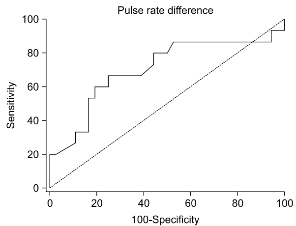
Figure 2. ROC curve of pulse rate change. Area under the ROC curve=0.704 (95% CI, 0.56 to 0.82). ROC: receiver operating characteristic; CI: confidence interval.
