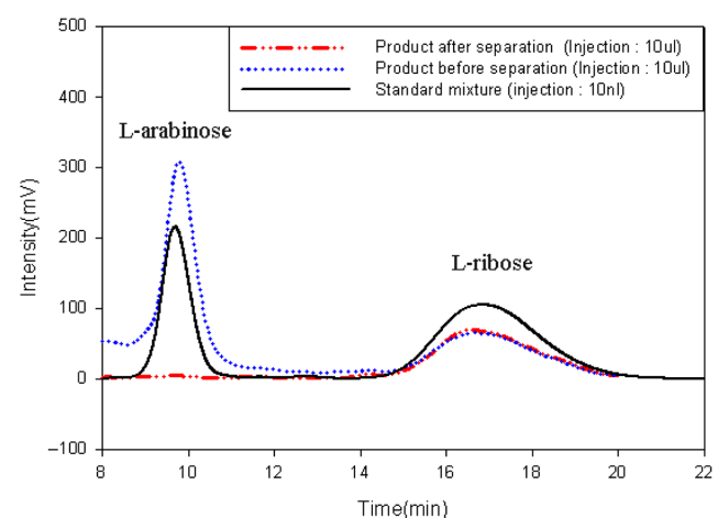
Fig. 2. Chromatograms of reaction mixture on SC 1011 HPLC column; temperature: 70 °C, flowrate: 1 mL/min, detector: UV, sample loading: 10 μL.
