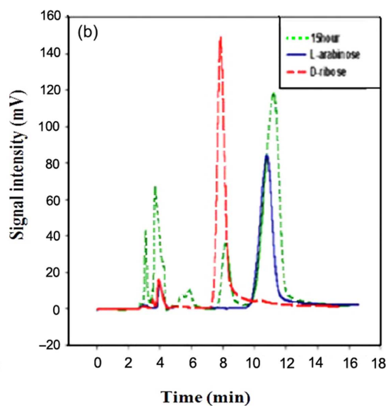
Fig. 5. Chromatograms of standard mixture (A) and reaction mixture after 15 hours (B) on Luna NH 2 column; temperature: 60 °C, flowrate: 1.0 mL/min, detector: UV, sample loop: 100 mL.
