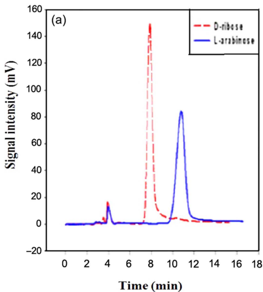
Fig. 5. Chromatograms of standard mixture (A) and reaction mixture after 15 hours (B) on Luna NH 2 column; temperature: 60 °C, flowrate: 1.0 mL/min, detector: UV, sample loop: 100 mL.
