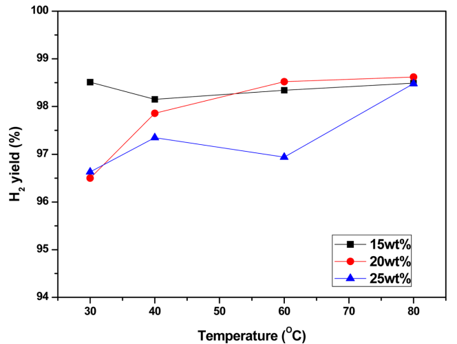
Fig. 6. The effect of temperature on the hydrogen yield of NaBH 4 hydrolysis reaction with NaBH 4 20 wt%.
