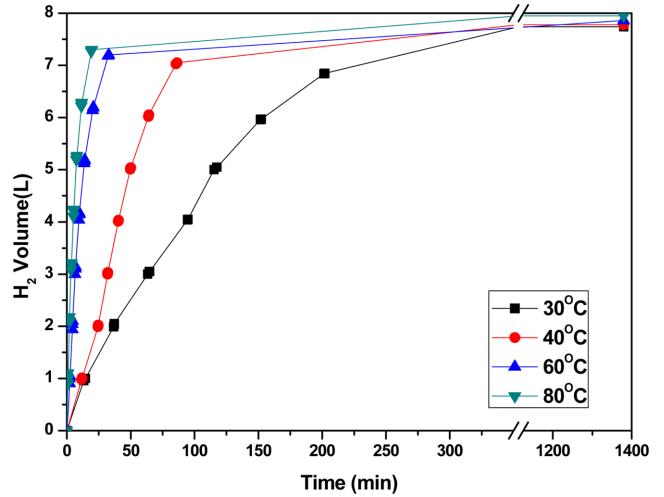
Fig. 5. The effect of temperature on the hydrogen evolution rate of NaBH 4 hydrolysis reaction with NaBH 4 20 wt%.
