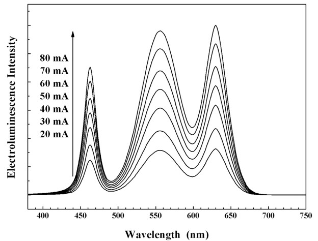
Fig. 4. Emission spectra of the Single-V device at various injection currents.
