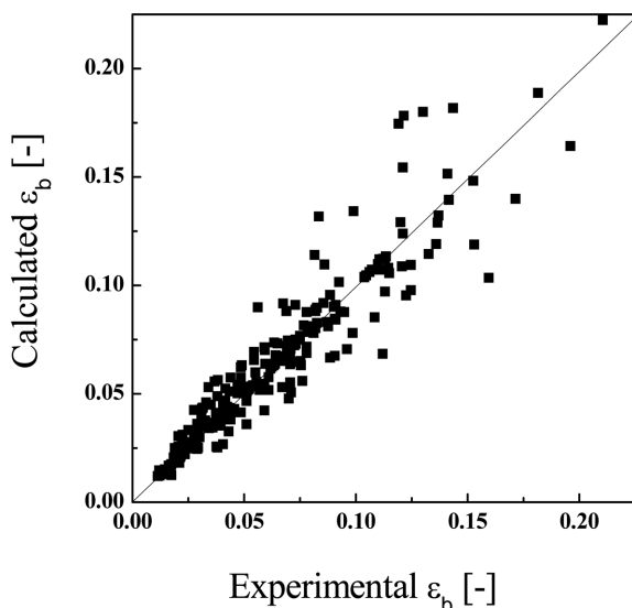
Fig. 9. Comparison of \epsilon_b values between the estimated and the experimentally obtained.
