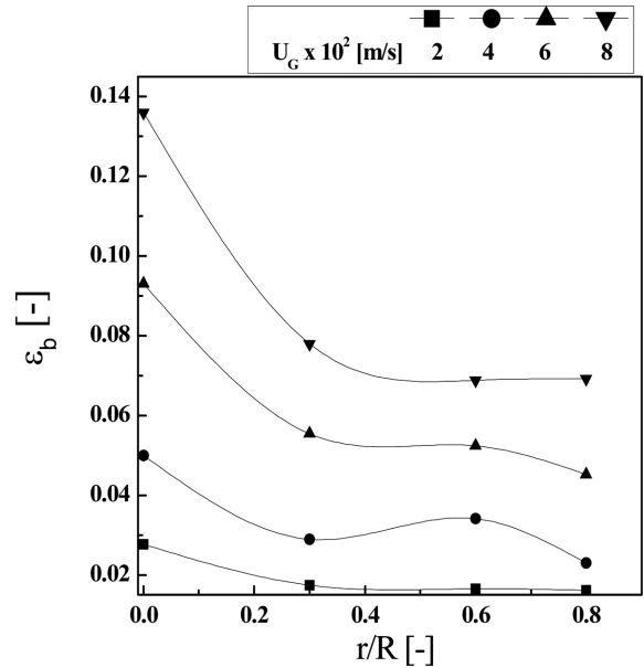
Fig. 3. Effects of gas velocity on the radial distribution of bubble holdup in a slurry bubble column reactor(H/L=0.35, σ L =0.072 N/m, S C =0.05).
