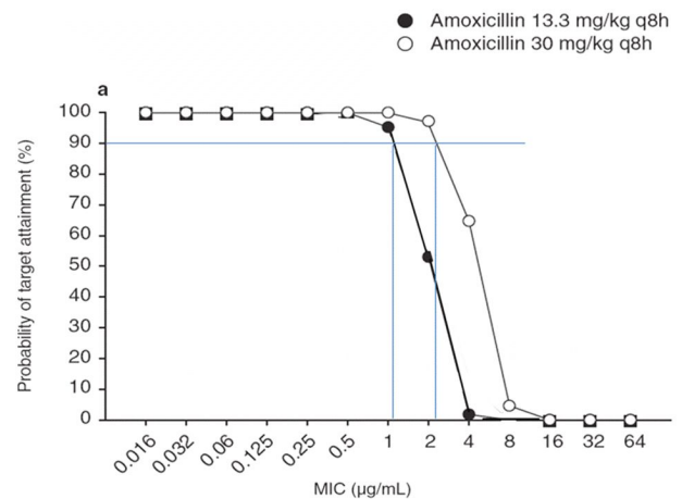
Fig. 1. Probability of target attainment for amoxicillin-based regimens achieving free drug concentrations above the MIC for 50% of the administration interval ( 50\% fT > MIC ) at increasing MIC dilutions 19) .
