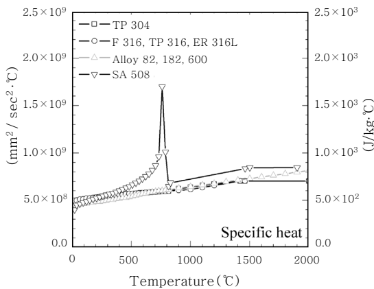
Fig. 6 Specific heat
