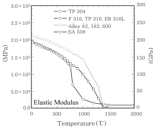
Fig. 10 Elastic modulus
