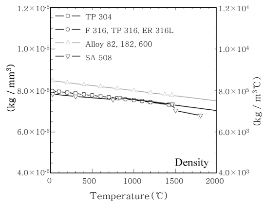
Fig. 8 Density
