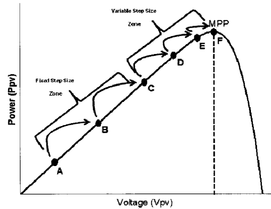
Fig. 3. Variable step size MPPT operation.
