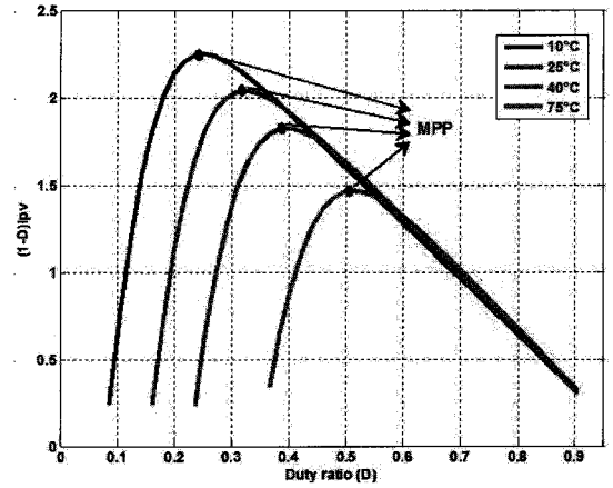
Fig. 6. Characteristic of the single current sensor MPPT with DC-DC boost converter at constant irradiation 1000 W/m².
