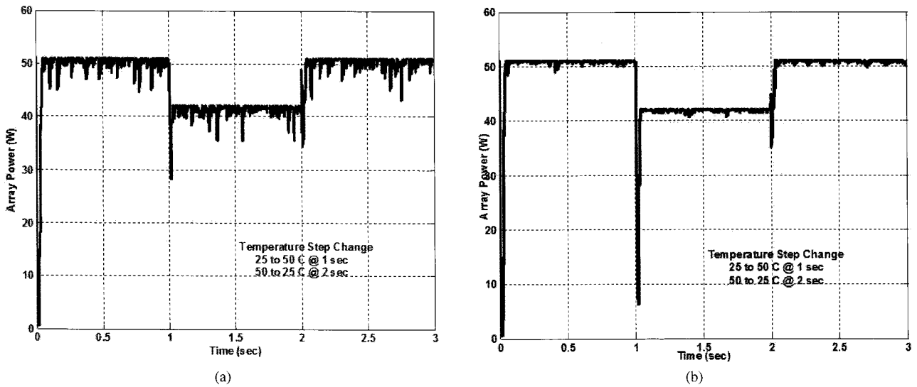
Fig. 12. Array power with the proposed variable step size MPPT due to Temperature Variation. (a) Method 1 ( M_1 = 0.025 ), (b) Method 2 ( M_2 = 0.5 ).
