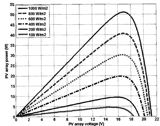
Fig. 1. Power-voltage characteristics of photovoltaic module at different irradiance levels with constant temperature (25°C).
