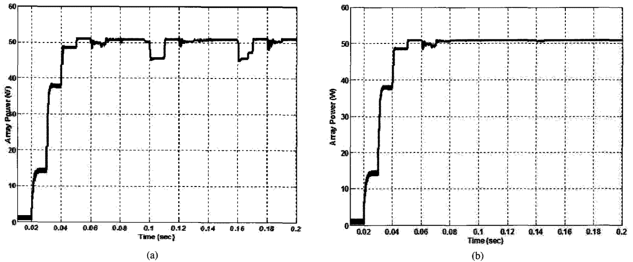
Fig. 9. Variable step size MPPT dynamic response with at a step change in the irradiation from 0 to 1000 W/m 2 . (a) Method 1 ( M_1 = 0.025 ), (b) Method 2 ( M_2 = 0.5 ).
