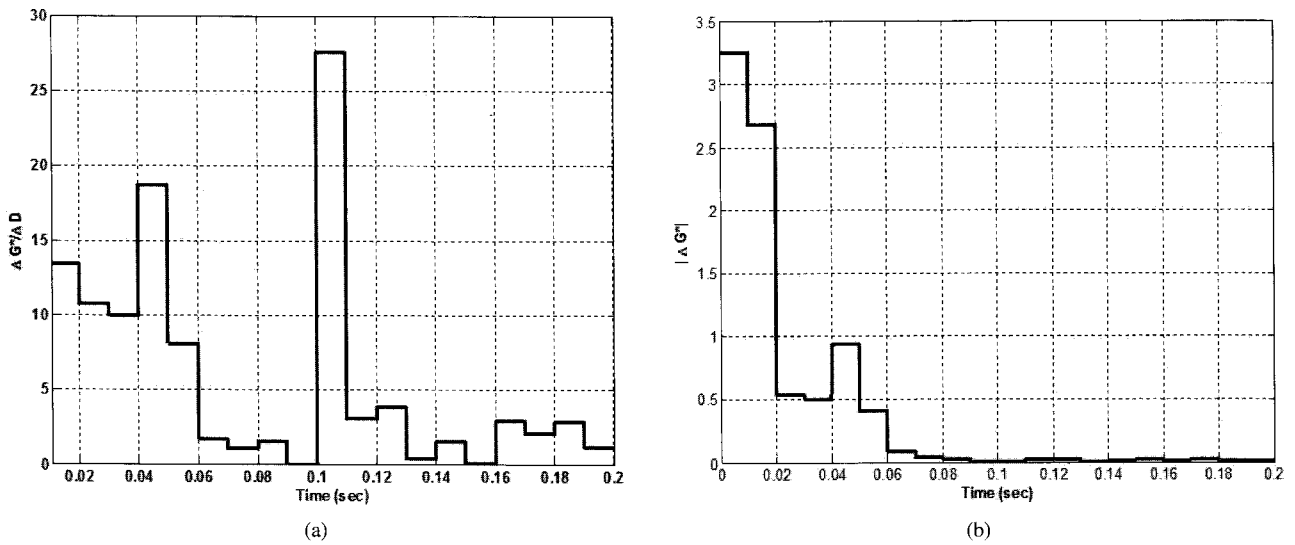
Fig. 11. Absolute value of the driving variable step size measure at a step change in the irradiation from 0 to 1000 W/m 2 . (a) Method 1 ( M_1 = 0.025 ), (b) Method 2 ( M_2 = 0.5 ).
