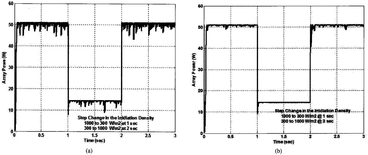
Fig. 14. Array power with the proposed variable step size. (a) Method 1 ( M_1 = 0.025 ), (b) Method 2 ( M_2 = 0.5 ).
