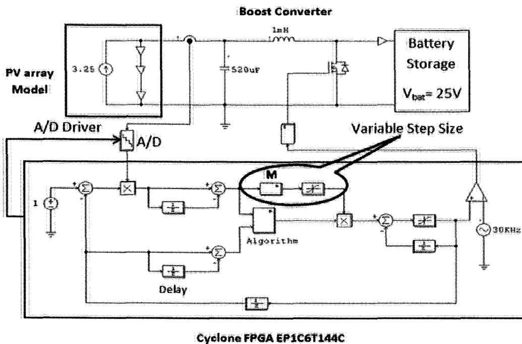
Fig. 8. Illustrative diagram of the hardware configuration equipped with a schematic diagram Of the proposed variable step size MPPT.
