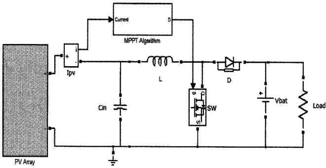
Fig. 4. Stand-alone single current sensor MPPT PV system equipped with DC-DC Boost converter.
