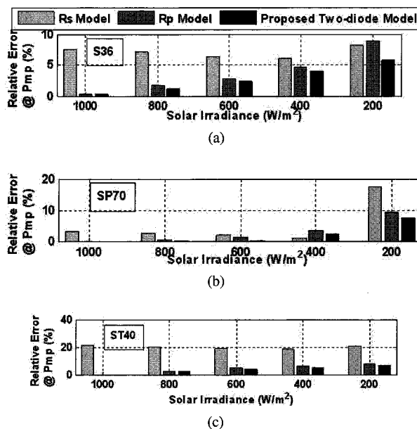
Fig. 15. Relative error for P_{mp} of R_s , R_p and the proposed two-diode model for irradiance variation. (a) S36. (b) SP70. (c) ST40.
