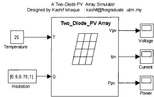
Fig. 7. PV simulator Block in Simulink.
