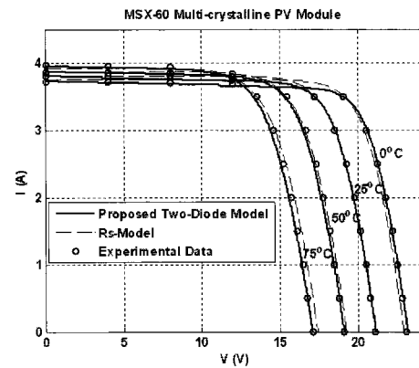
Fig. 11. I-V curves of R_s and proposed two-diode model of the MSX 60 PV module for several temperature levels @ 1\text{KW}/\text{m}^2 .
