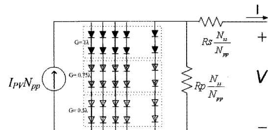
Fig. 18. A PV array illustration for the partial shading condition ( \lambda=1000\text{W/m}^2 ).
