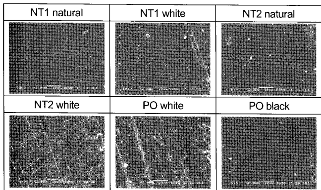
Figure 9. Surface morphologies by SEM analysis after exposing to \text{O}_2 plasma at 200 °C.
