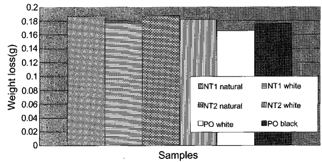
Figure 6. Comparison of weight losses after exposing to NF 3 to plasma at 300 °C.
