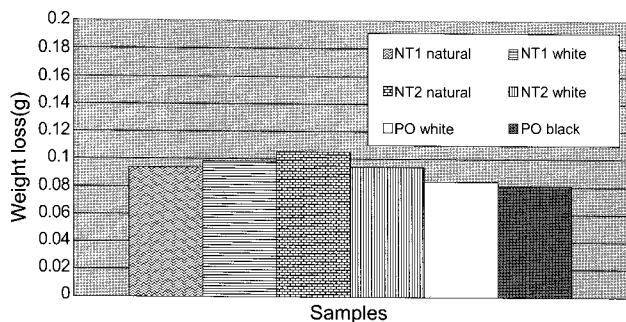
Figure 7. Comparison of weight losses after exposing to \text{O}_2/\text{NF}_3 plasma at 200 °C.
