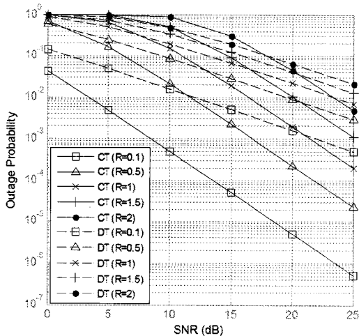
Fig. 2. Outage probability of cooperative and non-cooperative protocol as a function of SNR for symmetric network with different rate.
