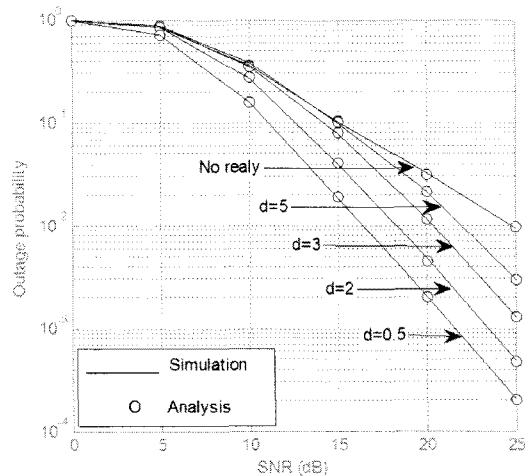
Fig. 6. Outage probability with different relay position.
