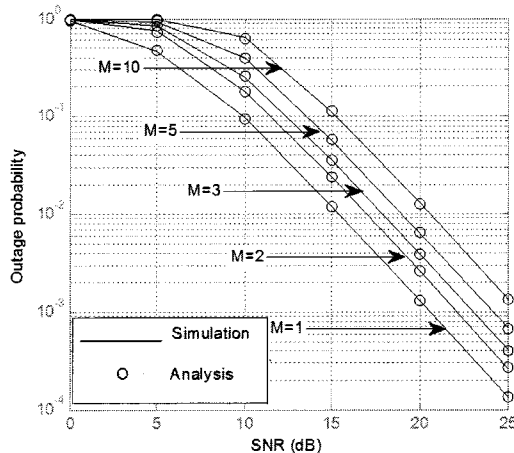
Fig. 3. Outage probability of symmetric network with R=1
