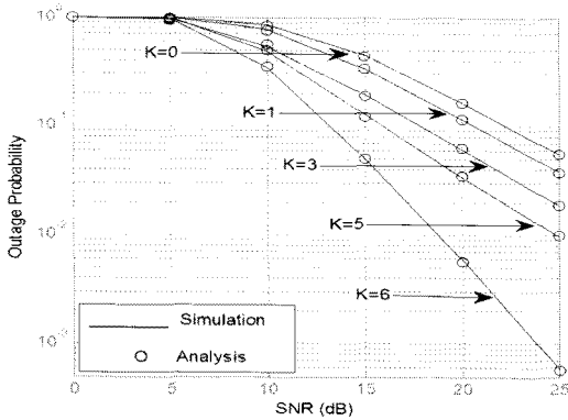
Fig. 5. Outage probability as a function of SNR for asymmetric network with different number of hop that selects a relay.
