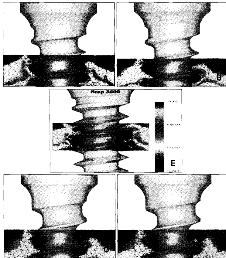
Fig 7. Radial strain development in the adjacent cortical bone at the final stage of self tapping microimplant placement of A, h200p6; B, h225p7; C, h250p8; D, h275p8; E, control models.
