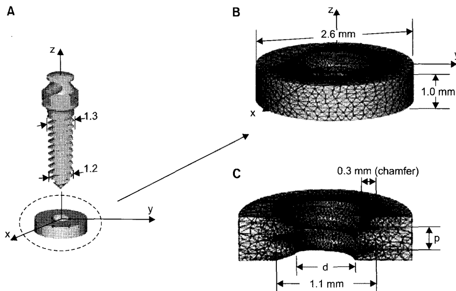
Fig 2. Geometry of microimplant and cortical bone specimen. A, Geometry model (unit: mm); B, shape and dimensional data of cortical bone specimen, constructed of tetrahedral elements; C, sectional view of cortical bone specimen, where p is the thread pitch for each of the 5 microimplants and d is the inner bone diameter made by the microimplant (0.7 mm and 0.9 mm for self drilling and self tapping simulations respectively).
