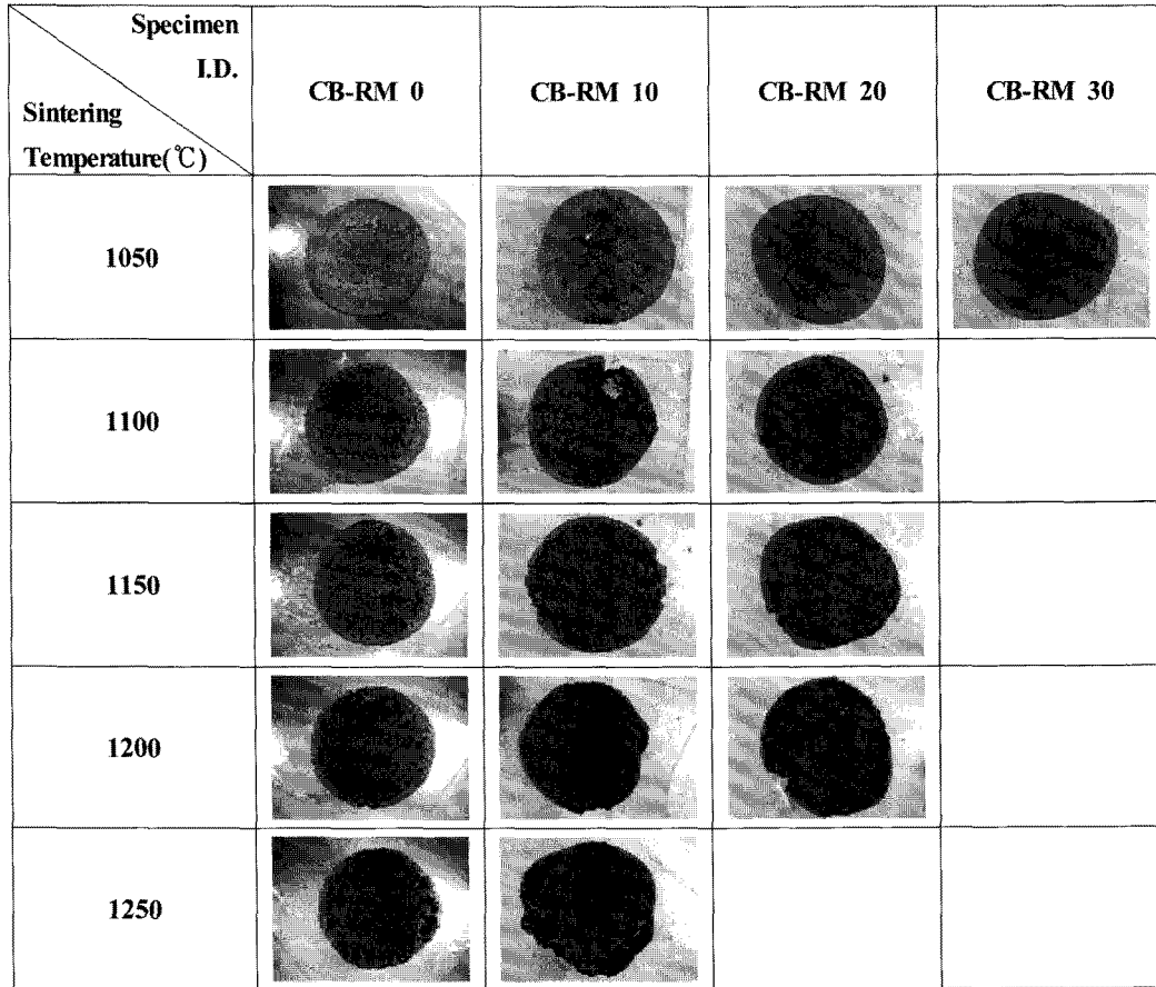
Fig. 6. Optical-microscopic photographs for the cut section of artificial aggregates sintered at 1050~1250°C for 10 min using direct sintering method in electric furnace.
