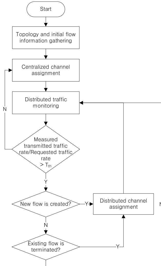
Fig. 1. Hybrid channel assignment procedure.
