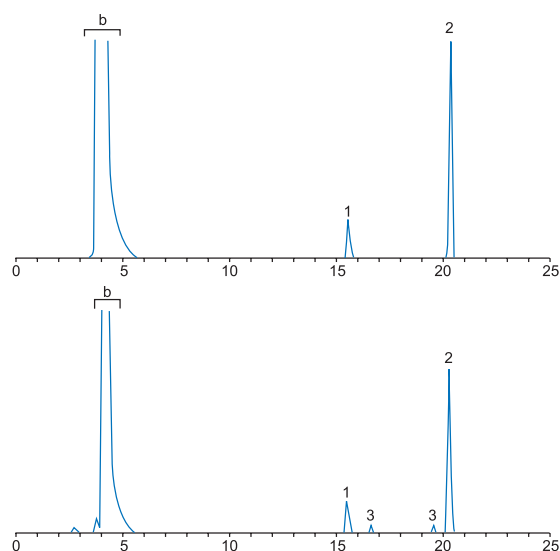
Figure 2. Chromatogram obtained from (A) standard solution and (B) urine according to the procedure for urine analysis.
