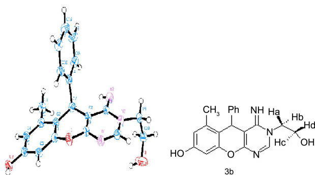
Fig. 1. X-ray Crystallographic Analysis. 3-(2-Hydroxyethyl)-4-imino-6-methyl-5-phenyl-4,5-dihydro-3H-chromeno[2,3-d]pyrimidin-8-ol, 3b.
