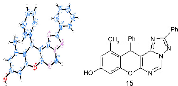
Fig. 2. X-ray Crystallographic Analysis. 11-Methyl-2,12-diphenyl-12H-chromeno[3,2-e][1,2,4]triazolo[1,5-c]pyrimidin-9-ol 15 .
