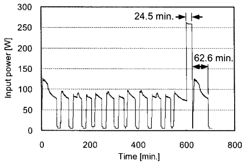
(a) Electric heater defrost
