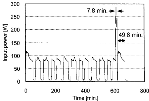
(b) Hybrid defrost
