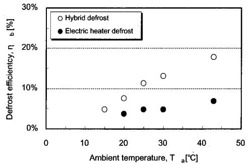
Fig. 8 Comparison of defrost efficiency between the hybrid defrost process and the electric heater defrost process.
