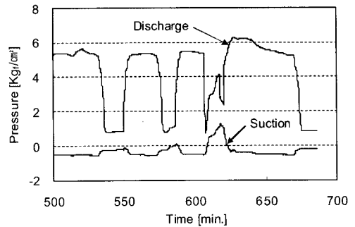
(a) Compressor pressure
