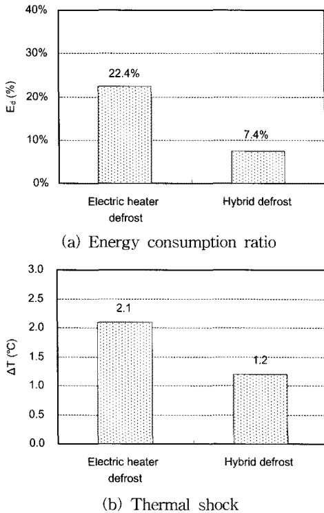
Fig. 9 Energy consumption ratio and thermal shock due to defrost heat in the hybrid defrost process and the electric heater defrost process.
