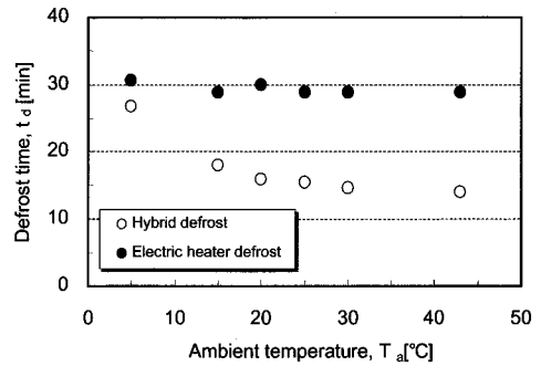
Fig. 7 Defrost time with ambient temperature.
