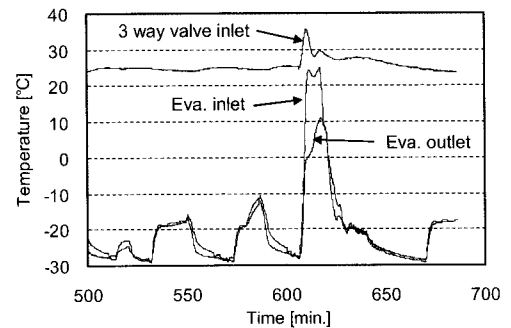
(b) Temperature of evaporator and valve
