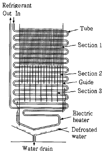
Fig. 1 Schematics of fin-tube heat exchanger.
