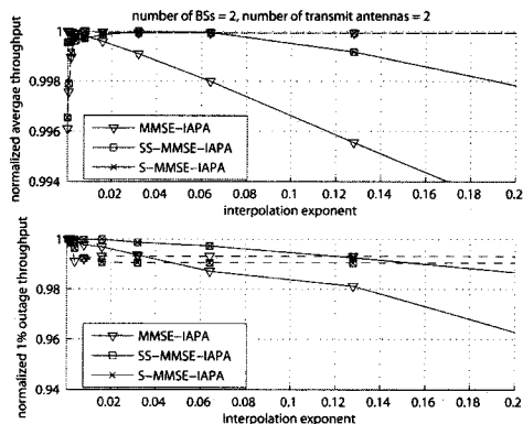
Fig. 5. Effect of the interpolation exponent on the average and 1% outage throughput (solid line : SNR = 0dB, dotted line : SNR = 20dB).
