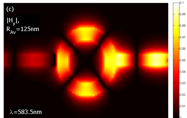
FIG. 4. (a) Transmittance spectrum of the simple band-pass plasmonic filter with circular ring resonator ( R_{Av} = 125 \text{ nm} , \Delta = 10 \text{ nm} ). (b) The |H_y| field profile of simple band-pass filter at the first resonance wavelength of \lambda = 1145 \text{ nm} . (c) The |H_y| field pattern of simple band-pass filter at the second resonance wavelength of \lambda = 583.5 \text{ nm} .
