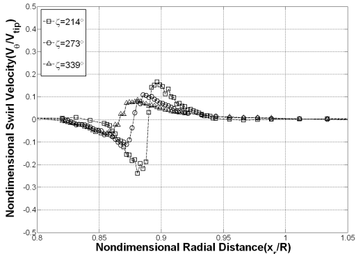
Fig. 3. Swirl velocity profiles
