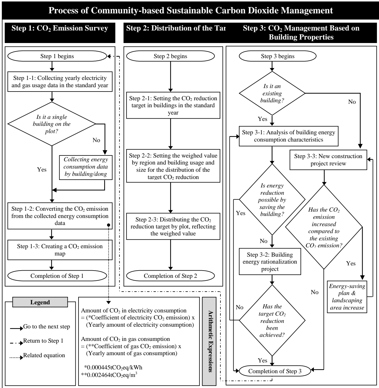
FIGURE II PROCESS OF COMMUNITY-BASED SUSTAINABLE CARBON DIOXIDE MANAGEMENT
