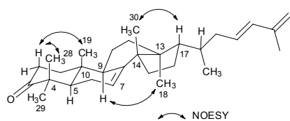
Figure 3. Important NOESY correlations for 1 .
