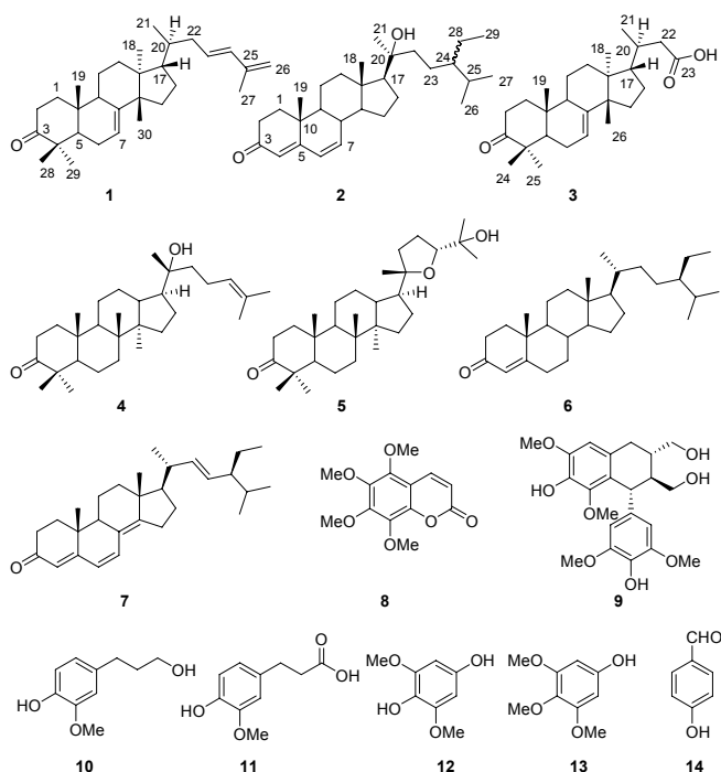
Figure 1. The structures of compounds 1-14.
