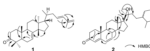
Figure 2. Important HMBC correlations for 1 and 2 .
