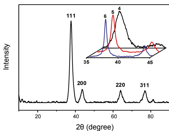
Figure 4. The XRD patterns of 6 . Inset shows the enlargements of the XRD patterns of 4 (black), 5 (red) and 6 (blue).
