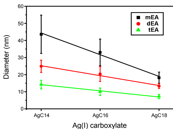
Figure 3. The relationship between the reductant, the chain length of the carboxylate ligand and the size of Ag NPs.
