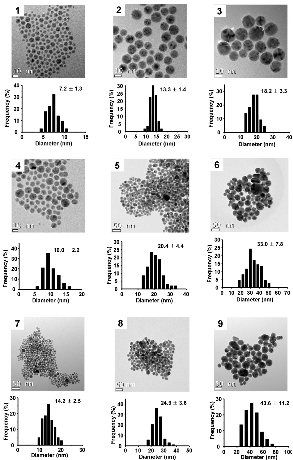
Figure 2. TEM images and the size distribution histograms of the Ag nanoparticles.
