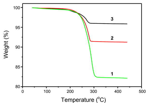
Figure 5. TGA curves of 1 (green), 2 (red) and 3 (black).
