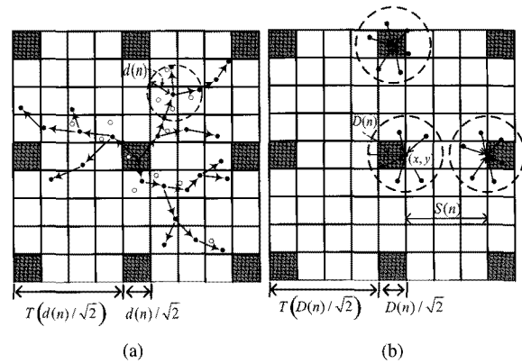
Fig. 2. a) Cell graph construction used to derive a lower bound on capacity. The solid dots are used to connect (n, m, m) cast tree while the blank dots are not part of the tree. b) TDMA scheme with decoding range D(n) . The parameter S(n) is defined to separate simultaneously communicating cells for successful communication condition based on physical model
