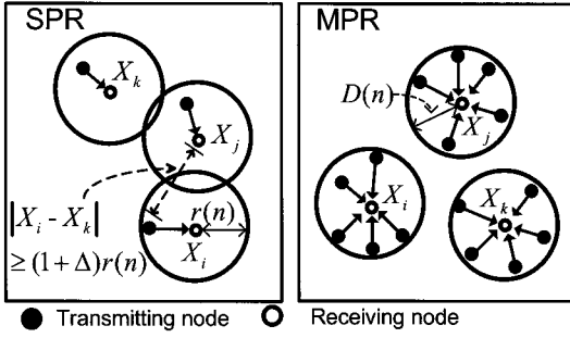
Fig. 1. Left figure describes the common successful transmission range r(n) for the protocol model [2] and right figure shows the common decoding range D(n) for MPR under the physical model. In this circular range, there are on average \pi n D^2(n) nodes.
