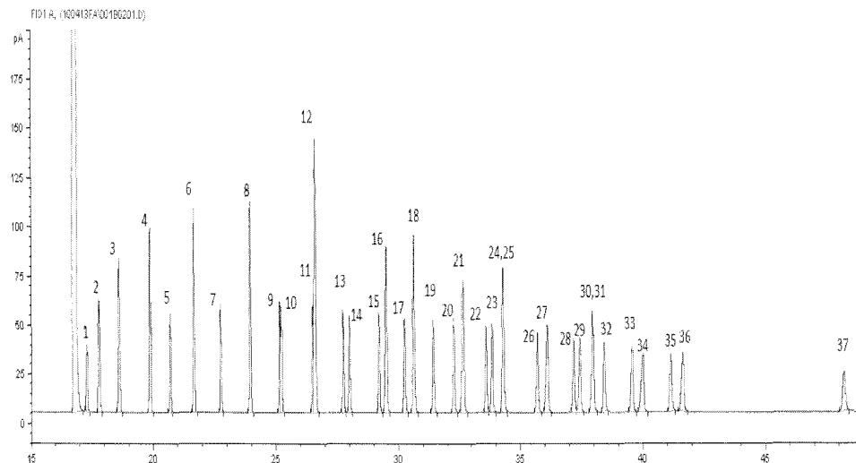
Fig. 1. GC chromatogram of 37 fatty acid standards.
