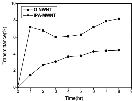
Figure 7. Transmittance of O-MWNT and IPA-MWNT solution.
