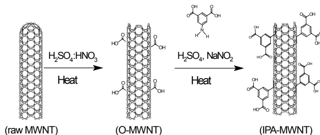
Figure 1. Surface modification of MWNT via the diazonium salt reaction.
