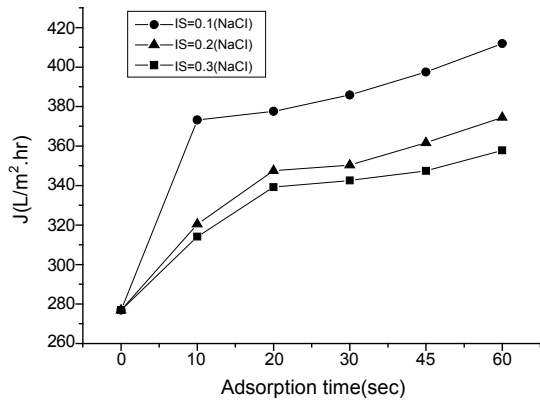
Figure 6. Effect of the ionic strength of NaCl and adsorption time in aqueous PSSA 1000 ppm solution on flux at room temperature.
