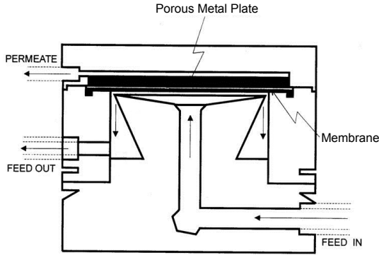
Figure 3. Schematic diagram of the membrane cell.
