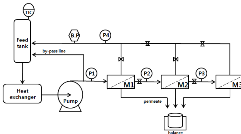
Figure 2. Experimental apparatus employed for the measurement of pure water permeability. P(1-4); pressure gauge, M(1-3); membrane cell, B.P.; back-pressure regulator, TIC; temperature indicator controller.
