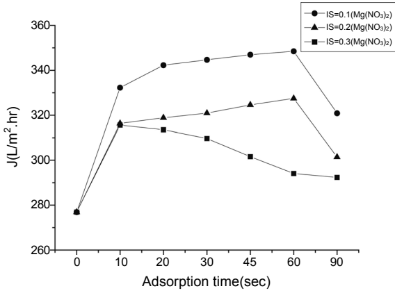
Figure 9. Effect of the ionic strength of Mg(NO_3)_2 and adsorption time in aqueous PSSA 1000 ppm solution on flux at room temperature.
