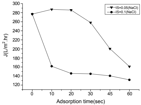
Figure 4. Effect of the ionic strength of NaCl and adsorption time in aqueous P(Am-co-AA) 1000 ppm solution on flux at room temperature.
