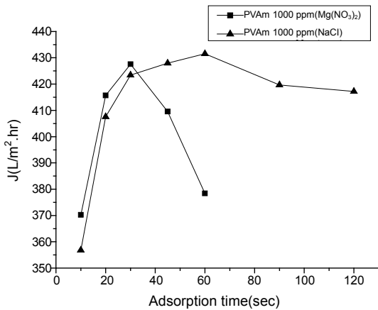
Figure 10. Effect of NaCl and Mg(NO_3)_2 salts and adsorption time in aqueous PVAm 1000 ppm solution at IS=0.1 and room temperature.
