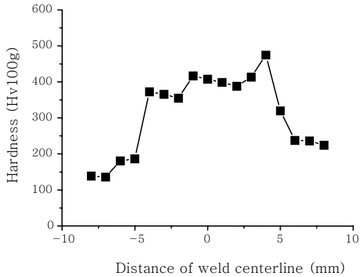
Fig. 9 Vickers hardness profile for annulus gear part
