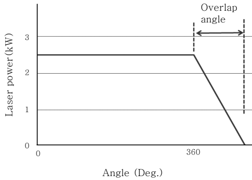
Fig. 5 Laser output power profile for crater elimination
