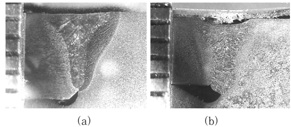
Fig. 8 Cross-sections: (a) annulus gear, (b) hub clutch assembly
