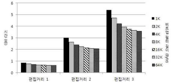
(a) DBLP-Author
