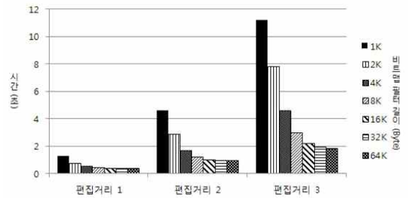
(b) DBLP-Title
