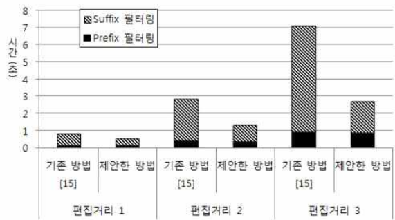
(b) DBLP-Title
