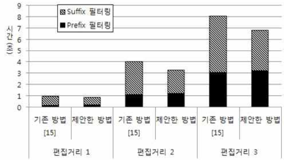
(a) DBLP-Author
