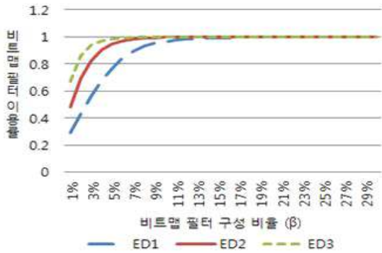
(a) DBLP-Author
