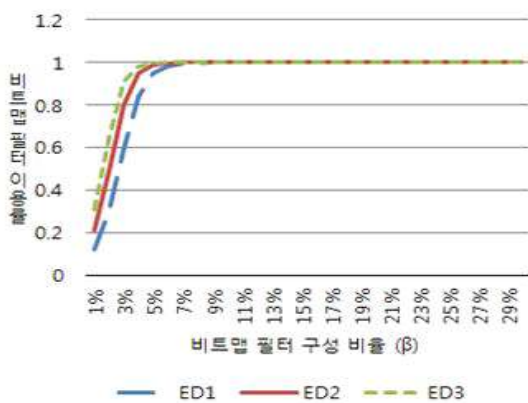
(b) DBLP-Title
