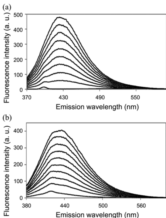
Figure 2. Fluorescence emission spectra of ANS (a) and TNS (b) in various concentrations of D2. [D2] = 0, 0.2, 0.4, 0.6, 0.8, 1.0, 1.2, 1.4, 1.6, 1.8 mM, [ANS] and [TNS] = 2.5 \mu M.
