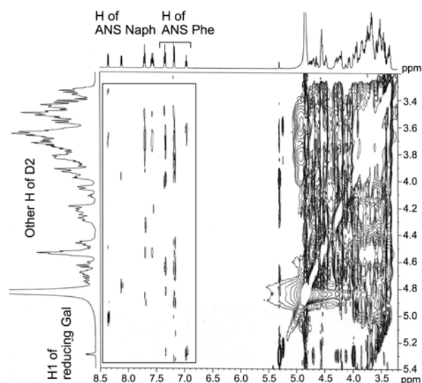
Figure 5. Partial NOESY spectrum of a D 2 O solution equimolar in ANS (14 mM) and D2 (14 mM). The rectangle contains the cross-peaks arising from the NOE interactions between protons of D2 and protons of ANS.
