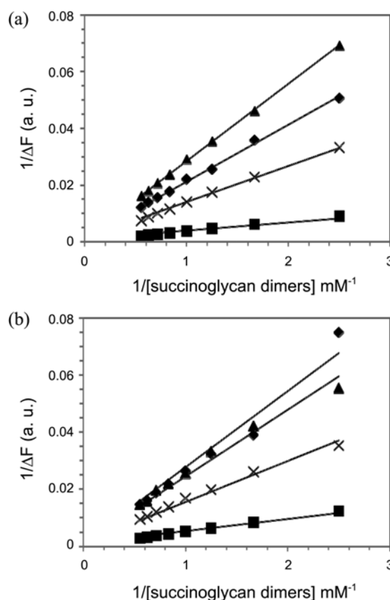
Figure 3. Double reciprocal plot of the concentration of succinoglycan dimers (D1; ◆, D2; ■, D3; ▲, D4; ×) and the increase in fluorescence intensity of ANS (a) and TNS (b).
