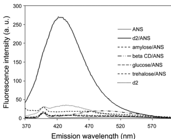
Figure 4. Emission spectra of ANS with other carbohydrates (amylose, \beta -CD, trehalose, and glucose) and D2 alone.
