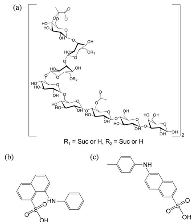
Figure 1. Chemical structures of succinoglycan dimers (a), ANS (b), and TNS (c). The succinoglycan dimers are classified with D1, D2, D3, and D4 according to the number of succinyl groups in the molecule.
