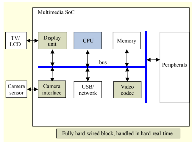
Fig. 2. Hardware platform of embedded multimedia SoC.
