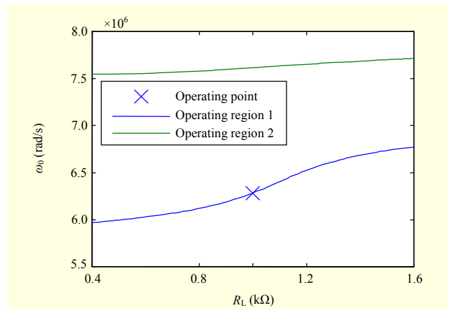
Fig. 5. \omega_0 with respect to R_L .
