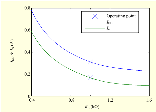
Fig. 7. I_{DD} and I_{o1m} with respect to R_L .
