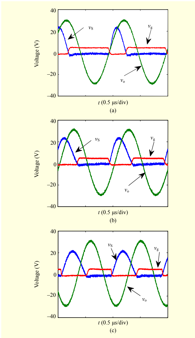
Fig. 9. Experiment waveform: (a) R_L=0.5 k \Omega , (b) R_L=1 k \Omega , and (c) R_L=1.5 k \Omega .
