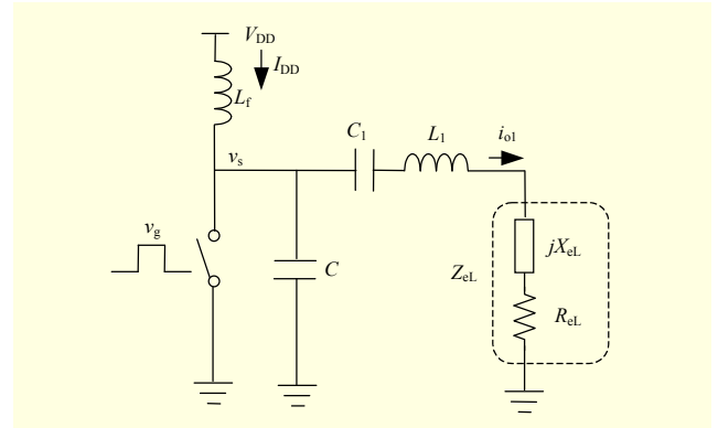
Fig. 2. Schematic diagram of the primary circuit with a reflected back resistance.
