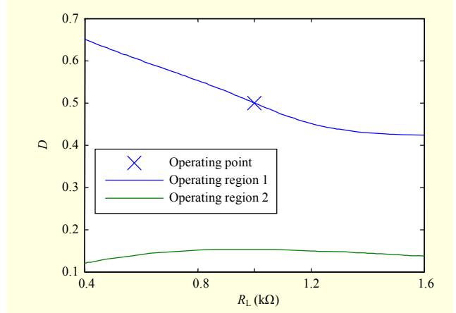
Fig. 4. D with respect to R_L .
