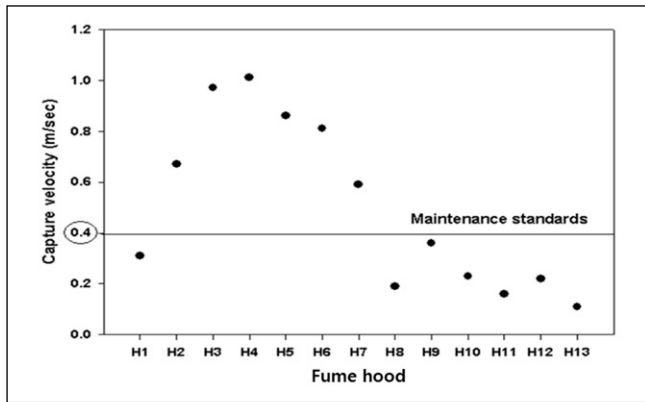
Fig. 4. Capture velocity of fume hoods in the laboratories.
