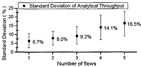
Fig. 12 Standard Deviation of Analytical Throughput on Multiple Flows
