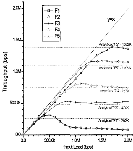
Fig. 11 Results of Scenario with Multiple Flows and Multiple Gateways
