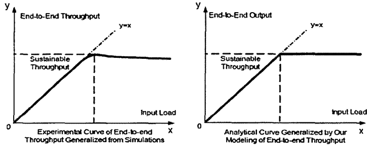
Fig. 5 End-to-end Throughput of Flows (Simulation v.s. Modeling)
