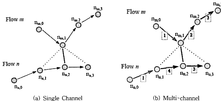
Fig. 2 Modeling Multi-flow and Multi-channel Scenarios
