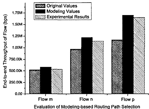
Fig. 14 Throughput Comparison of Modeling-based Route Selection Method
