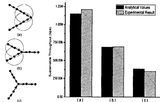
Fig. 9 Topology and Simulation Results of Joint Flows
