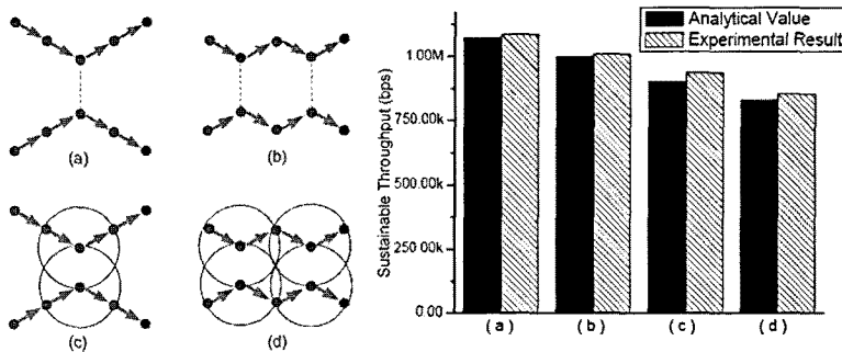
Fig. 7 Topology and Simulation Results of Two Flows
