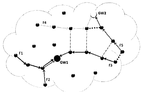
Fig. 10 Scenarios with Multiple Flows and Multiple Gateways
