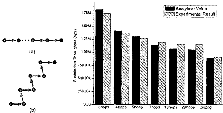
Fig. 6 Topology and Simulation Results of Single Flow
