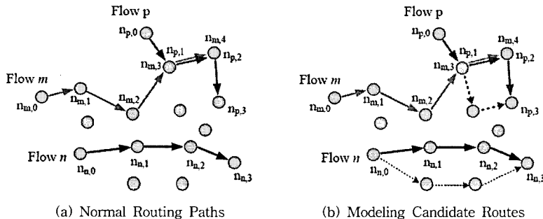
Fig. 4 Example of Modeling-based Route Selection
