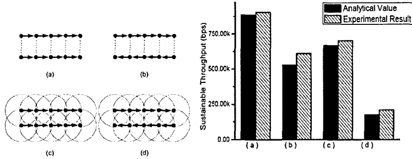
Fig. 8 Topology and Simulation Results of Parallel Flows
