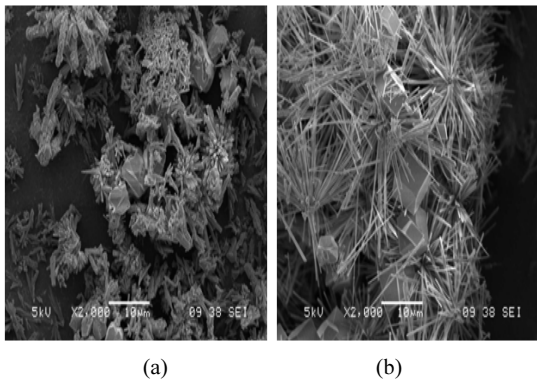
[그림 2] SEM image of Calcium carbonate by adding EDTA 0.00625g/L (a) 40℃, (b) 60℃
