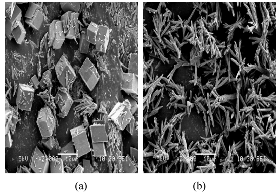
[그림 4] SEM image of Calcium carbonate by adding DTPA 0.00625g/L (a) 40℃, (b) 60℃
