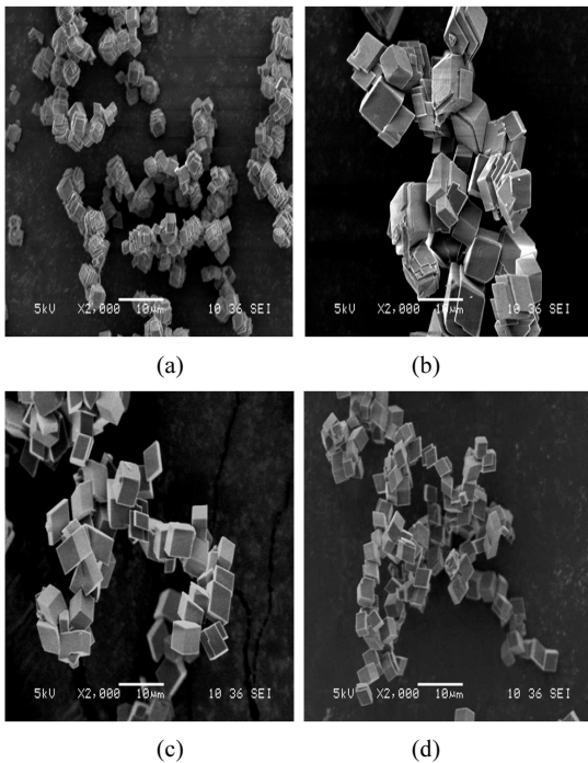
[그림 7] SEM image of Calcium carbonate by adding PMA 0.00625g/L (a) 20°C, (b) 40°C, (c) 60°C, (d) 80°C
