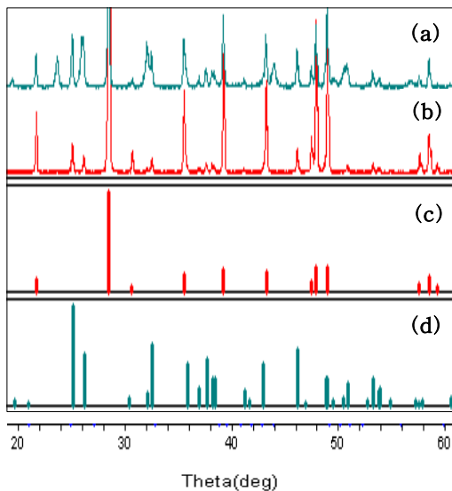
[그림 3] XRD results of Calcium carbonate by adding EDTA 0.00625g/L (a) 40℃, (b) 60℃, (c) calcite library, (d) aragonite library
