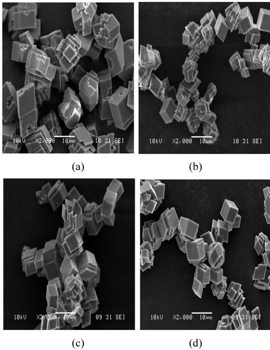
[그림 6] SEM image of Calcium carbonate by adding CIT 0.00625g/L (a) 20°C, (b) 40°C, (c) 60°C, (d) 80°C
