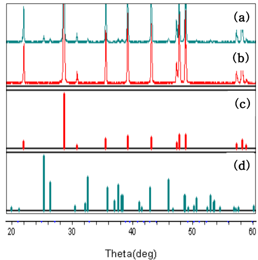
[그림 5] XRD results of Calcium carbonate by adding DTPA 0.00625g/L (a) 40℃, (b) 60℃, (c) calcite library, (d) aragonite library
