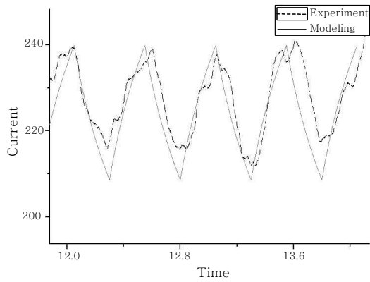
Fig. 3 Welding current waveform for 3mm root gap and 45° groove angle
