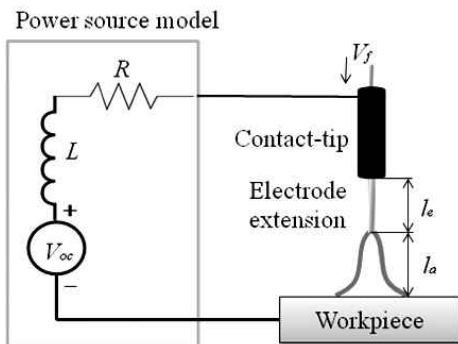
Fig. 1 P-GMA welding system
