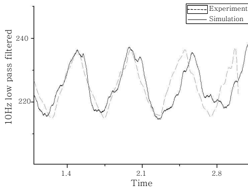
Fig. 10 Welding current waveform for 3mm root gap and 60° groove angle after model modification with weld pool
