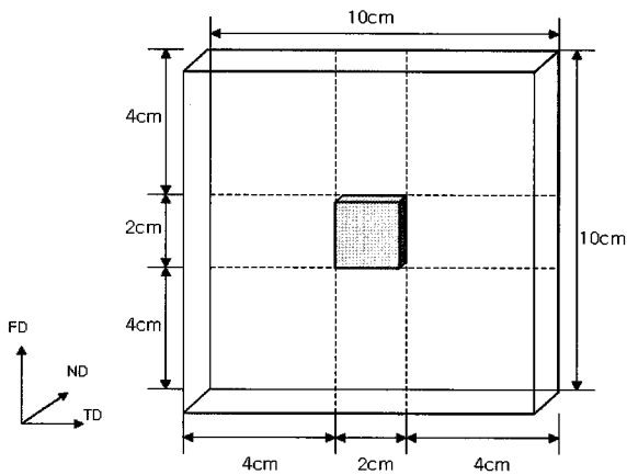
Figure 3. A specimen with the size of 2 cm×2 cm cut 4 cm away from the edge of HVIS specimens for a morphology analysis.
