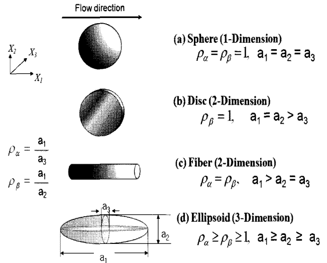
Figure 2. Schematic views of inclusions with the shape of a sphere (a); disc (b); fiber (c); ellipsoid (d) with their orientation relative to sample axes.
