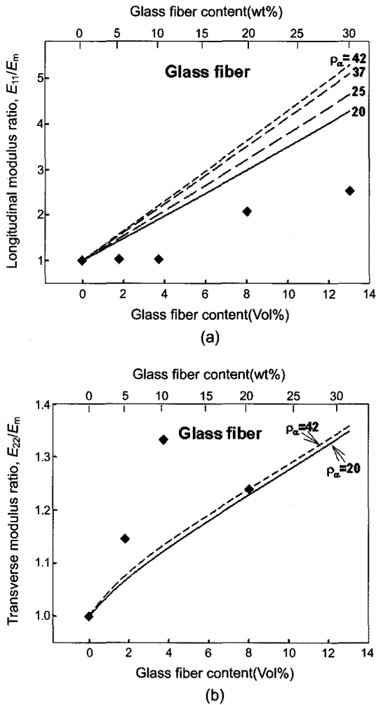
Figure 8. Comparison of longitudinal Young's modulus ratio, E_{11}/E_m (a); transverse Young's modulus ratio, E_{22}/E_m (b) of experimental data with theoretical prediction as a function of the content of glass fiber.
