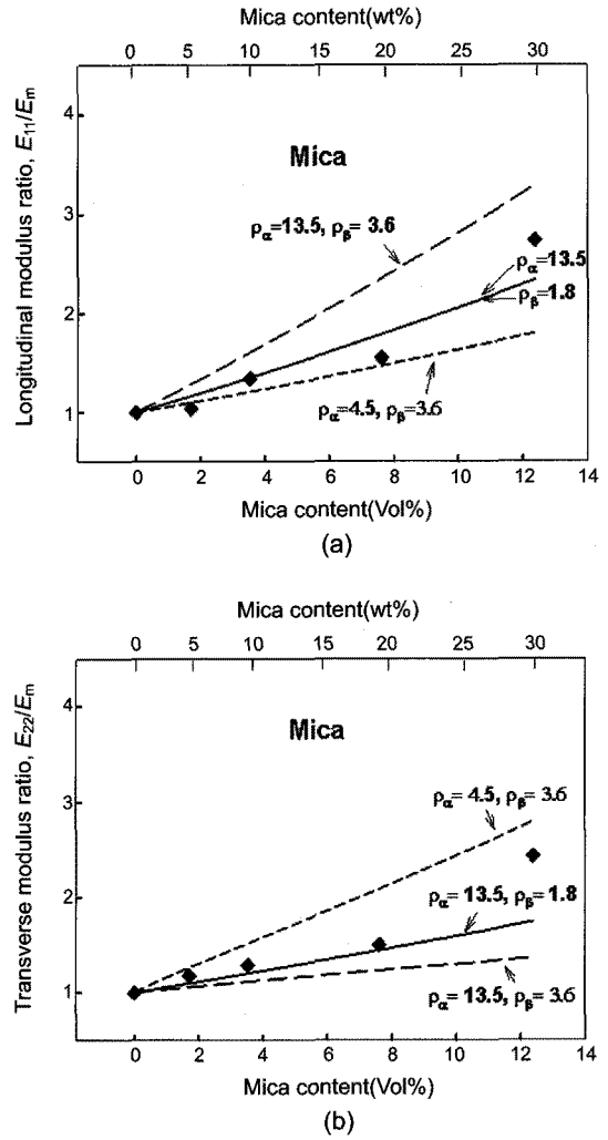
Figure 9. Comparison of longitudinal Young's modulus ratio, E_{11}/E_m (a); transverse Young's modulus ratio, E_{22}/E_m (b) of experimental data with theoretical prediction as a function of the content of mica.
