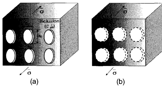
Figure 1. A composite formed from aligned ellipsoidal inclusions ( a_1 > a_2 > a_3 ) with two aspect ratio.
