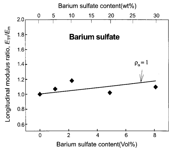
Figure 7. Comparison of longitudinal Young's modulus ratio, E_{11}/E_m , of experimental data with the theoretical prediction as a function of the content of barium sulfate.
