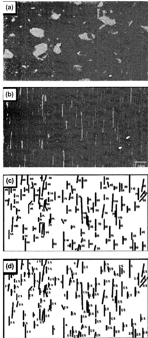
Figure 5. Image of SEM for the PP/composites filled with 10 wt% of mica parallel to ND (a); parallel to FD (b); schematic illustration of the length (μm) (c); thickness(μm) (d).
