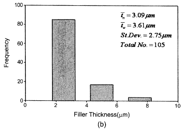
Figure 6. Histogram of mica filler length (a); filler thickness (b) in PP/mica composites.
