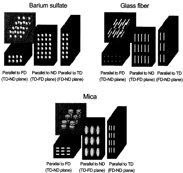
Figure 4. Schematic view of the alignment of filler in the composites as a view point.
