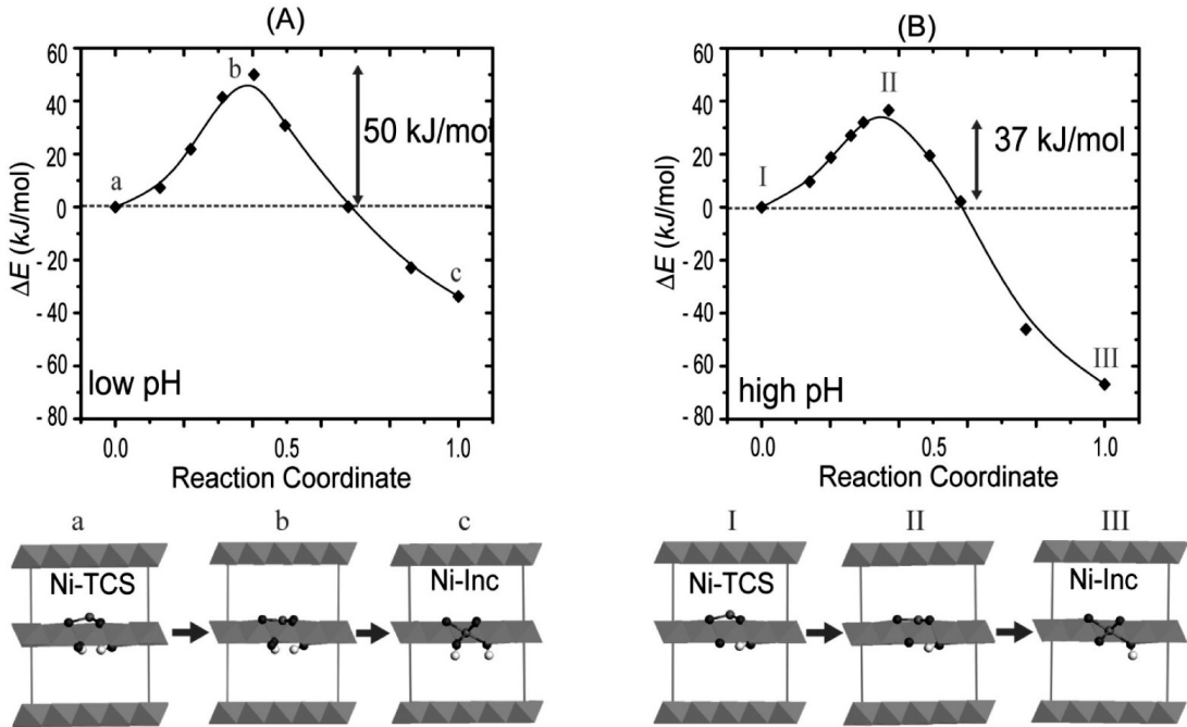
Fig. 3. Comparison of the relative activation energy from Ni-TCS to Ni-Inc reaction at (a) low pH and (b) high pH. The b and II represent the transition state in (A) and (B), respectively. Figure reproduced by permission of Elsevier, from Peña et al. (2010).
