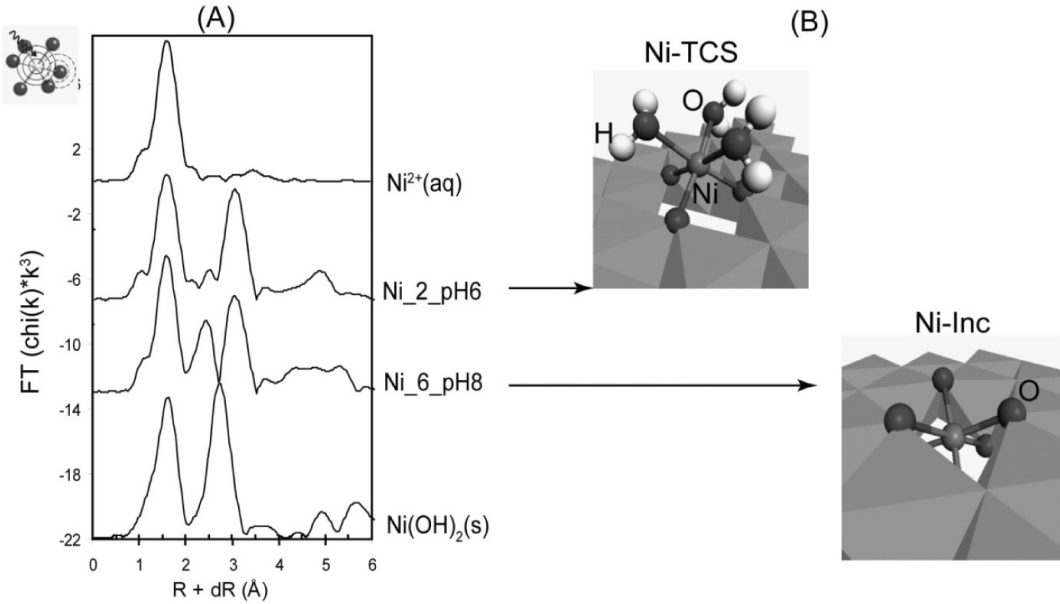
Fig. 2. (A) Fourier transforms of Ni K-edge EXAFS spectra for aqueous Ni, Ni-adsorbed bacteriogenic birnessite, and Ni(OH) 2 (from Peña et al. , 2010). (B) Molecular structures of main Ni species at a Mn(IV) vacancy, corresponding to each sorption pH condition guided by arrows. Ni-TCS: Ni triple-corner-sharing surface complex above the vacancy; Ni-Inc: Ni incorporated inside the vacancy. Polyhedra represent edge-sharing MnO 6 octahedra.
