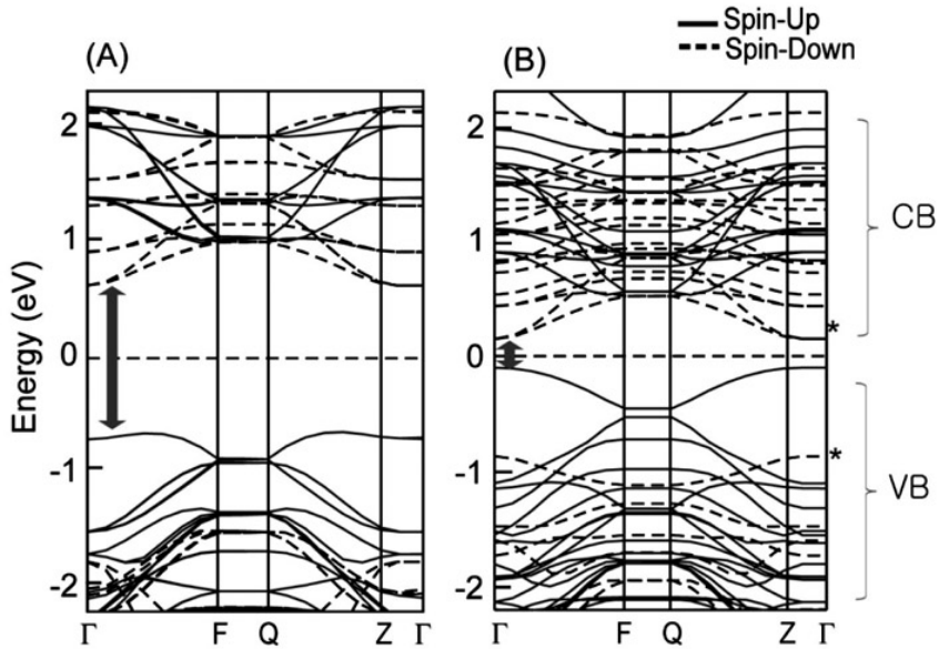
Fig. 4. Calculated band structures of (A) vacancy-free hexagonal layer-type MnO 2 and (B) MnO 2 with 12.5% Mn(IV) vacancies (each vacancy was charged-compensated with four h). Double-headed arrows indicate the band gap. Solid and dashed lines are energy bands for spin-up and spin-down electrons, respectively. CB: conduction band; VB: valence band. X-axis represents high-symmetry points which electron wavevectors take on in the first Brillouin zone. Asterisks(*) in (B) show a direct band gap for spin-down electrons at the \Gamma point. Figure reproduced by permission of APS, from Kwon et al. (2008).
