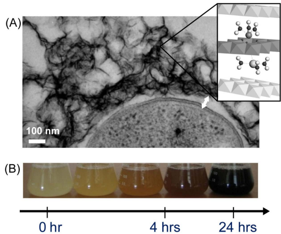
Fig. 1. (A) Transmission electron microscopic image of cross-section of Pseudomonas putida GB-1 cell and Mn oxide particles precipitated outside the cell. The inset figure represents the part of the biogenic Mn oxide crystal structure, where hydrated Mn(III) and Na^+ cations charge-balance a Mn(IV) vacancy. (B) Photograph of P. putida GB-1 culture showing the fast kinetics in bacterial oxidation of Mn(II) into oxide particles, at an initial rate of 140 \pm 5 \mu Mh^{-1} (Peña, 2009). The culture at 0 hour corresponds to the stationary phase of the cell growth. The electron microscopic image and the culture photo are from Peña (2009).
