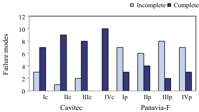
Fig. 5. Comparison of failure modes of zirconia crowns with different coping design and cement type. Ic, IIc, IIIc, IVc means group I, II, III, IV in Cavitec ® Subgroup, Ip, IIp, IIIp, IVp means group I, II, III, IV in Panavia-F ® subgroup.
