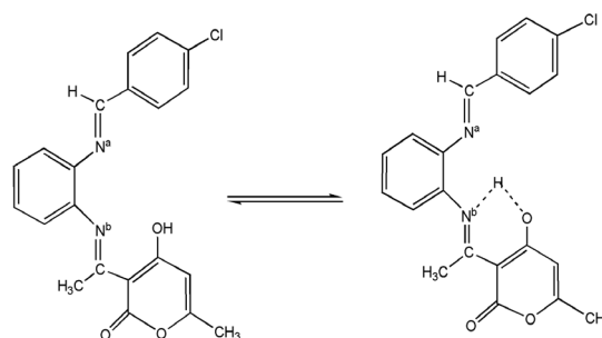
Fig. 2. Resonance structure of the ligand.
