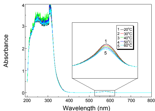
Fig. 2. Absorption spectra of the closed forms of 1.0 \times 10^{-3} M Blue 502 in MeOH solution. The inset shows the absorption spectra with extended scales of the closed forms in the ranges between 520 nm and 620 nm.
